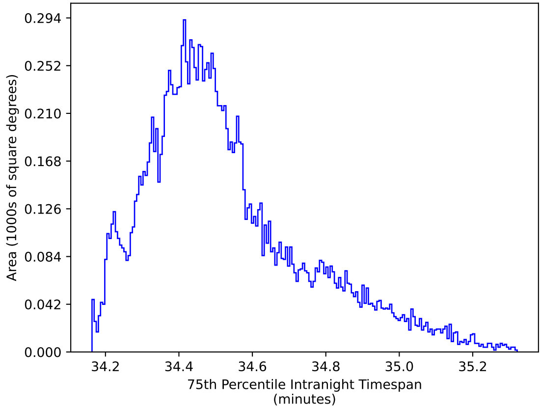
roll_uniform_eh_acc0.2_mjdp0_v3.4_10yrs WFD zy bands: 75th Percentile Intranight Timespan
