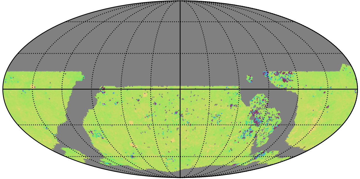
roll_uniform_eh_acc0.2_mjdp0_v3.4_10yrs WFD ug bands: 75th Percentile Intranight Timespan
