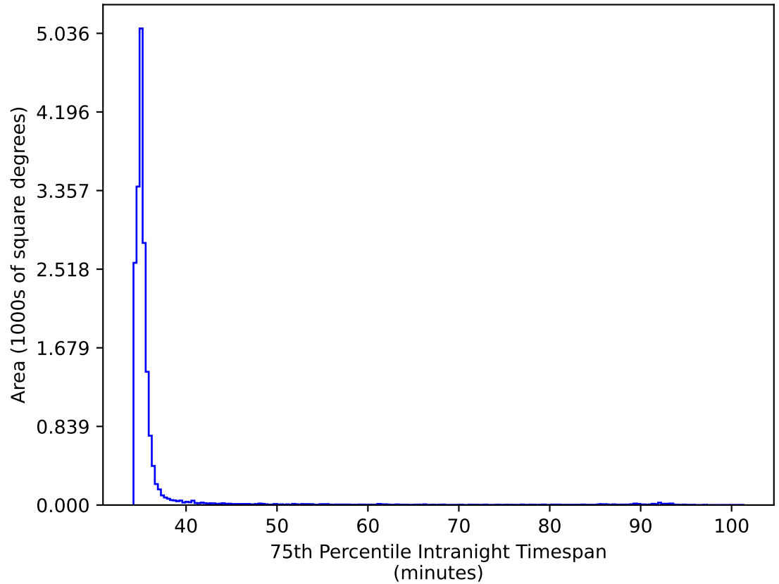
roll_uniform_eh_acc0.2_mjdp0_v3.4_10yrs WFD ri bands: 75th Percentile Intranight Timespan
