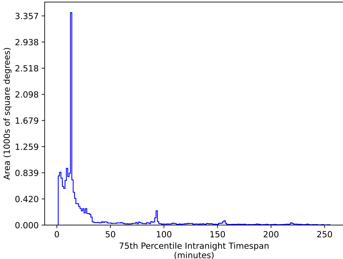
roll_uniform_eh_acc0.2_mjdp0_v3.4_10yrs WFD i band: 75th Percentile Intranight Timespan
