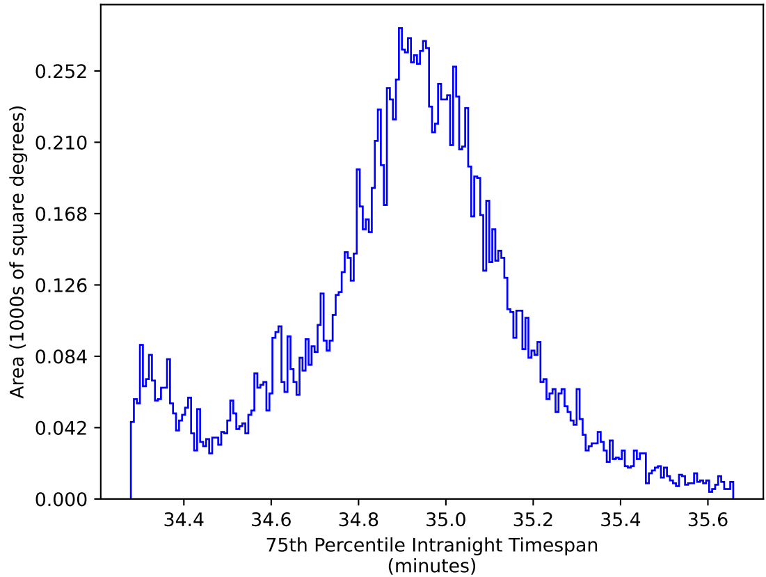
roll_uniform_eh_acc0.2_mjdp0_v3.4_10yrs WFD all bands: 75th Percentile Intranight Timespan
