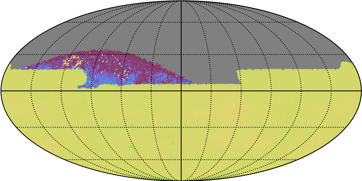
roll_uniform_eh_acc0.2_mjdp0_v3.4_10yrs All sky zy bands: 75th Percentile Intranight Timespan
