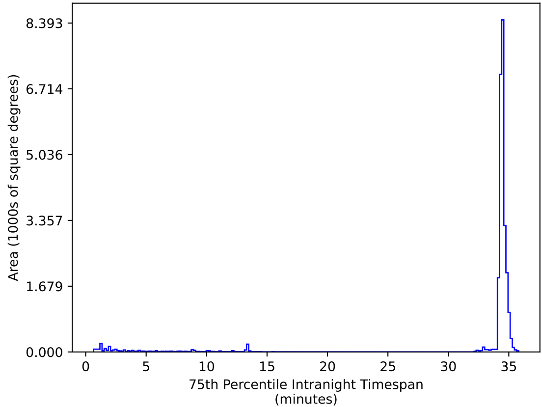
roll_uniform_eh_acc0.2_mjdp0_v3.4_10yrs All sky zy bands: 75th Percentile Intranight Timespan
