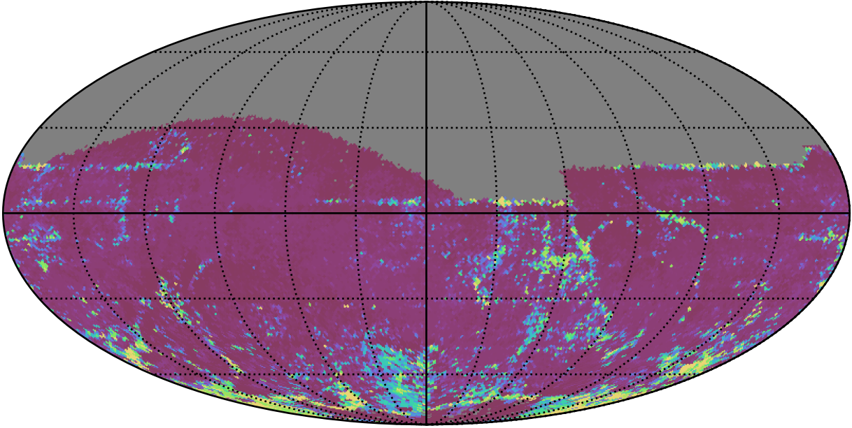
roll_uniform_eh_acc0.2_mjdp0_v3.4_10yrs All sky z band: 75th Percentile Intranight Timespan
