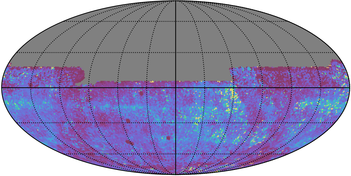
roll_uniform_eh_acc0.2_mjdp0_v3.4_10yrs All sky y band: 75th Percentile Intranight Timespan
