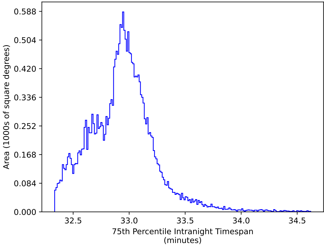
roll_uniform_eh_acc0.2_mjdp0_v3.4_10yrs All sky y band: 75th Percentile Intranight Timespan
