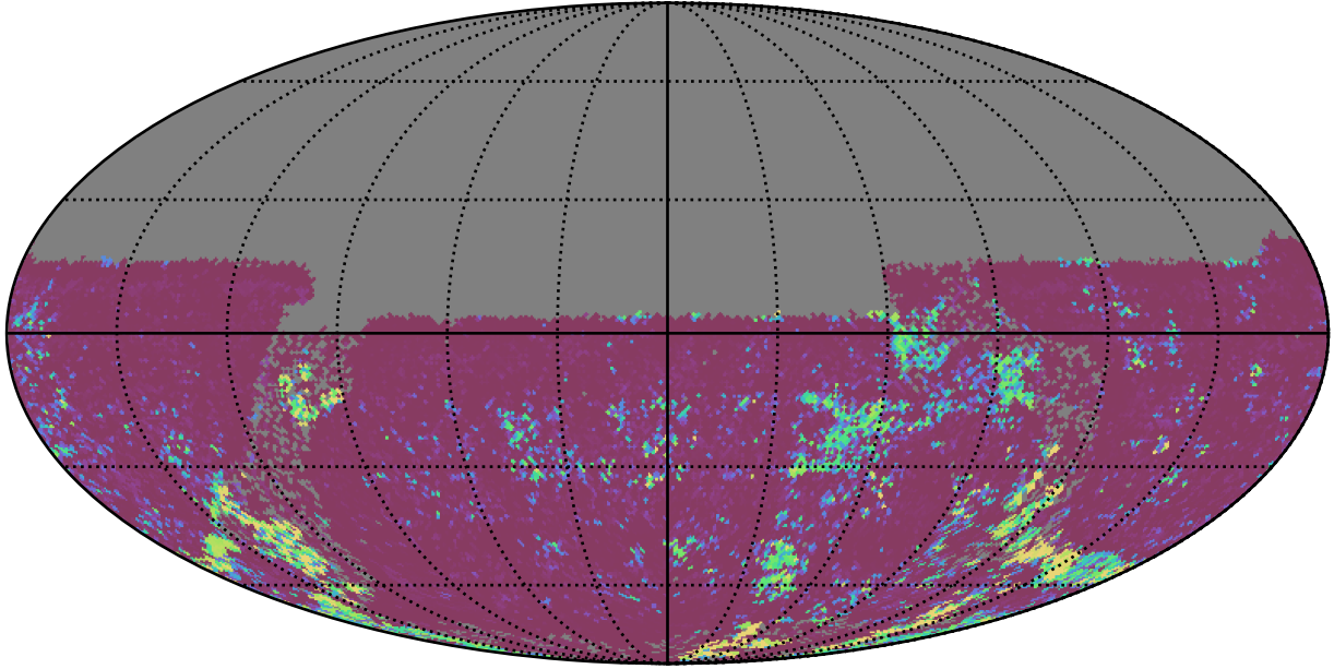
roll_uniform_eh_acc0.2_mjdp0_v3.4_10yrs All sky u band: 75th Percentile Intranight Timespan
