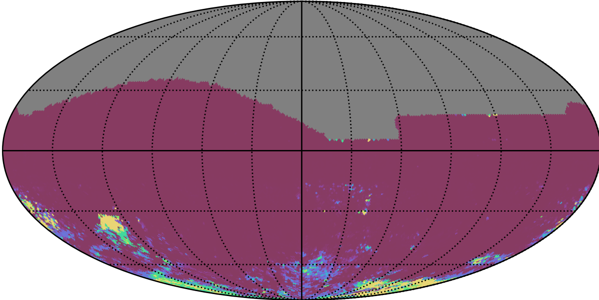
roll_uniform_eh_acc0.2_mjdp0_v3.4_10yrs All sky ri bands: 75th Percentile Intranight Timespan
