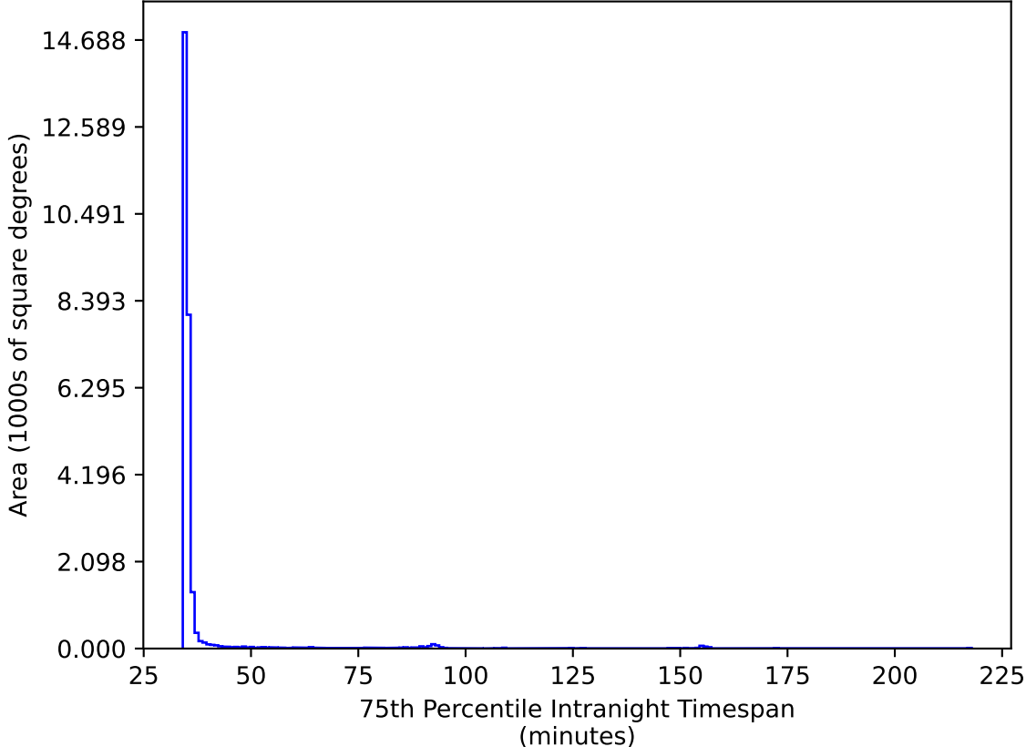
roll_uniform_eh_acc0.2_mjdp0_v3.4_10yrs All sky ri bands: 75th Percentile Intranight Timespan
