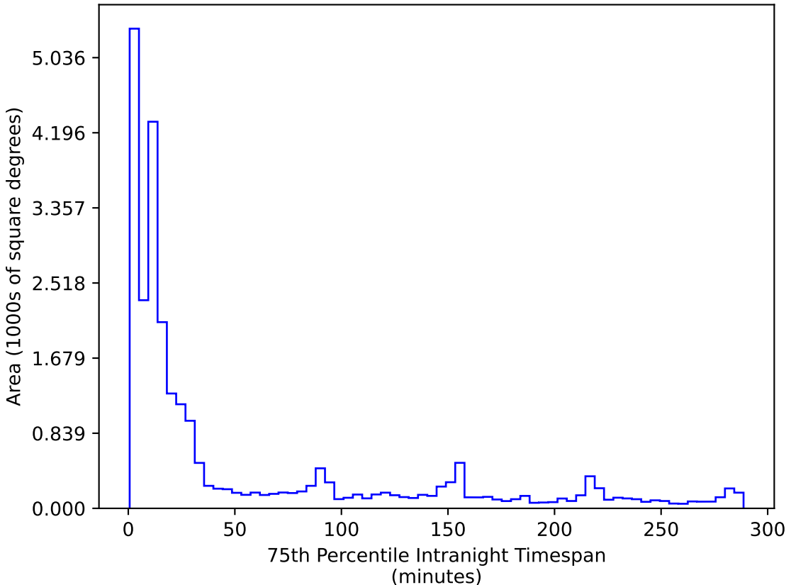
roll_uniform_eh_acc0.2_mjdp0_v3.4_10yrs All sky r band: 75th Percentile Intranight Timespan
