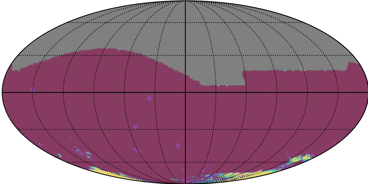
roll_uniform_eh_acc0.2_mjdp0_v3.4_10yrs All sky iz bands: 75th Percentile Intranight Timespan
