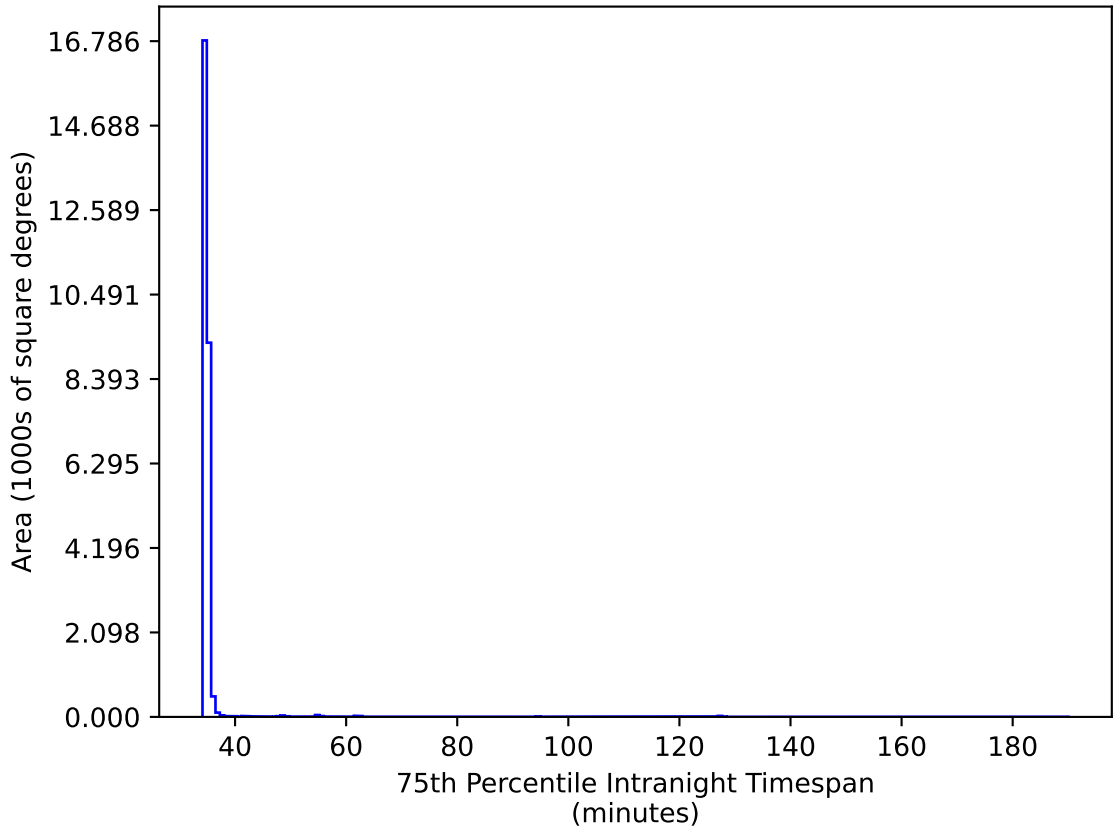
roll_uniform_eh_acc0.2_mjdp0_v3.4_10yrs All sky iz bands: 75th Percentile Intranight Timespan
