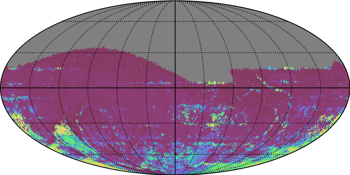
roll_uniform_eh_acc0.2_mjdp0_v3.4_10yrs All sky i band: 75th Percentile Intranight Timespan
