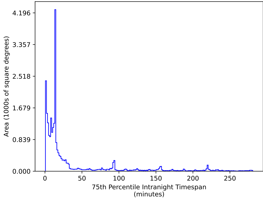
roll_uniform_eh_acc0.2_mjdp0_v3.4_10yrs All sky i band: 75th Percentile Intranight Timespan
