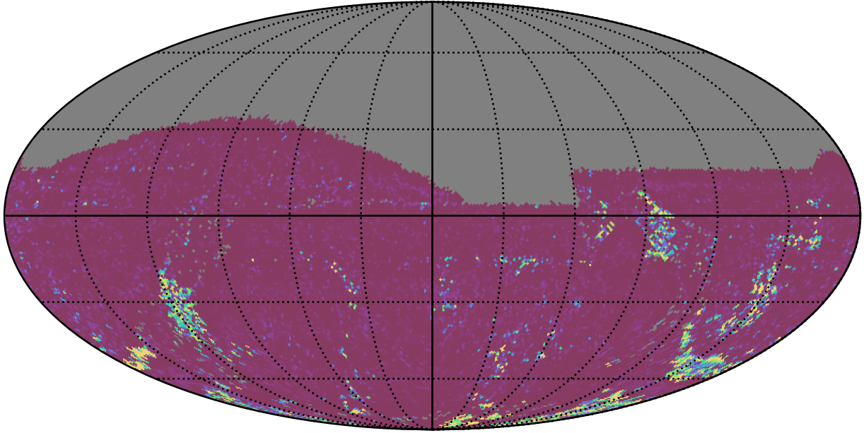
roll_uniform_eh_acc0.2_mjdp0_v3.4_10yrs All sky g band: 75th Percentile Intranight Timespan
