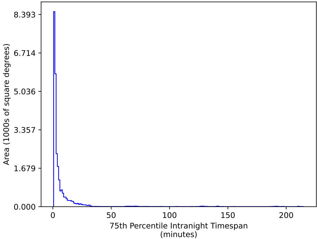
roll_uniform_eh_acc0.2_mjdp0_v3.4_10yrs All sky g band: 75th Percentile Intranight Timespan
