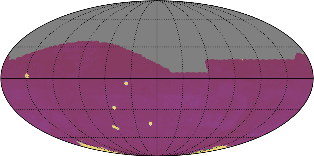
roll_uniform_eh_acc0.2_mjdp0_v3.4_10yrs All sky all bands: 75th Percentile Intranight Timespan
