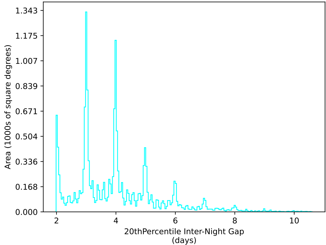
roll_uniform_eh_acc0.2_mjdp0_v3.4_10yrs WFD u band: 20thPercentile Inter-Night Gap
