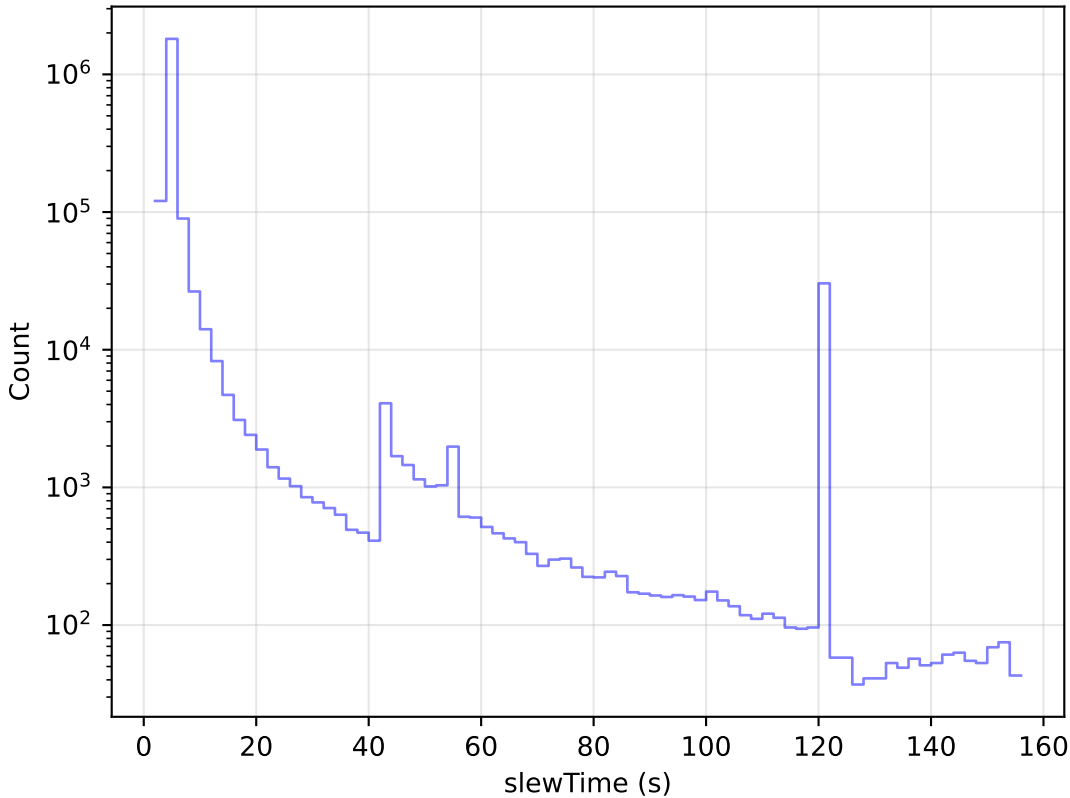
roll_uniform_eh_acc0.2_mjdp0_v3.4_10yrs All visits: Slew Time Histogram
