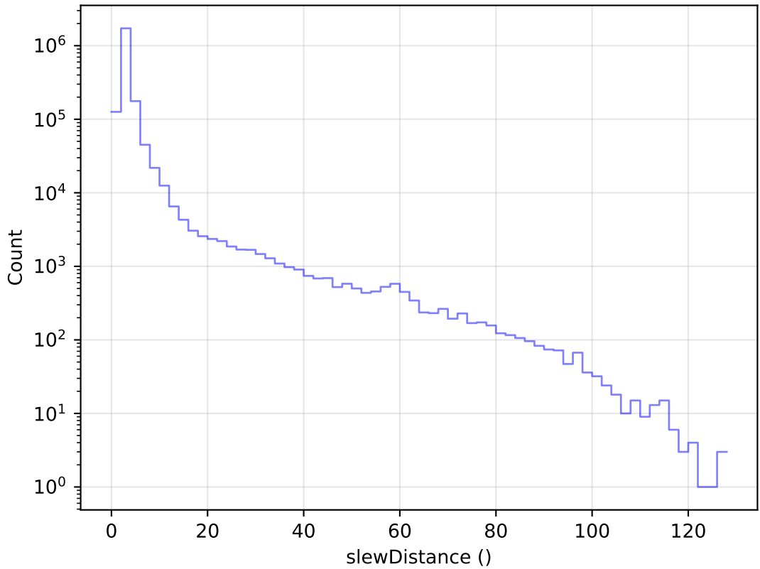
roll_uniform_eh_acc0.2_mjdp0_v3.4_10yrs All visits: Slew Distance Histogram
