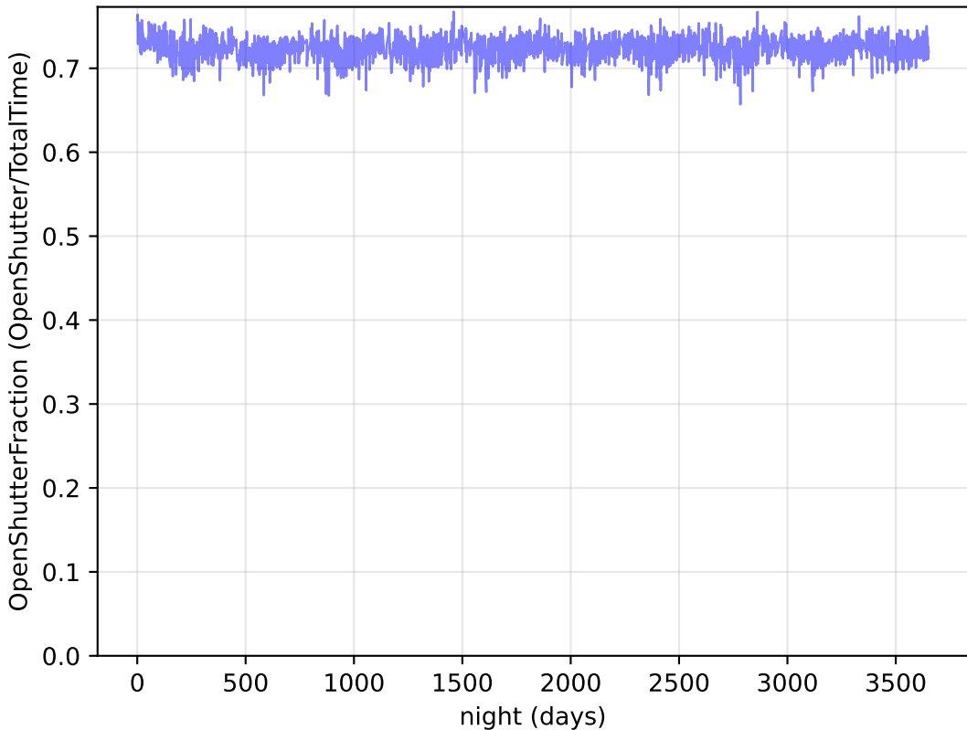
roll_uniform_eh_acc0.2_mjdp0_v3.4_10yrs : OpenShutterFraction
