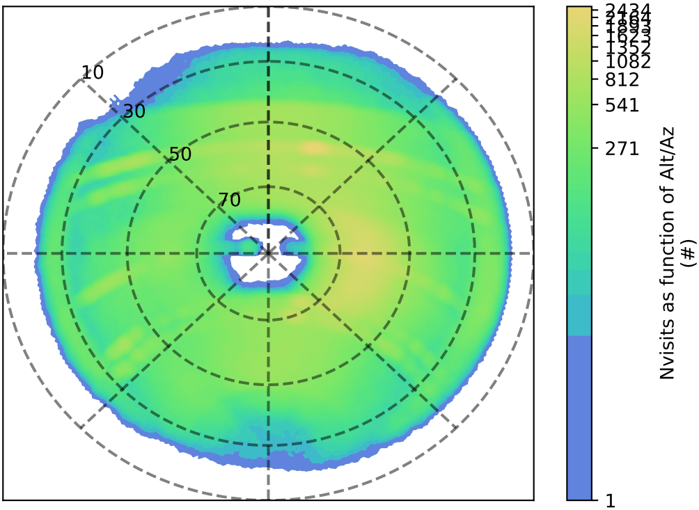
roll_uniform_eh_acc0.2_mjdp0_v3.4_10yrs z: Nvisits as function of Alt/Az
