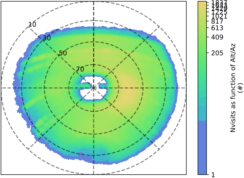
roll_uniform_eh_acc0.2_mjdp0_v3.4_10yrs y: Nvisits as function of Alt/Az
