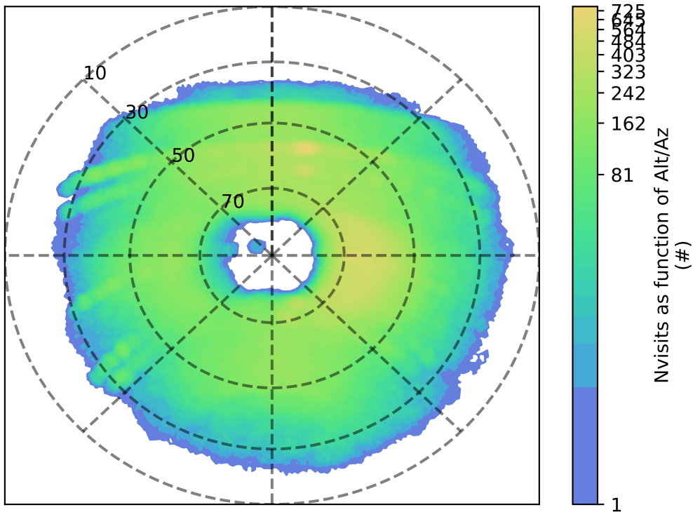
roll_uniform_eh_acc0.2_mjdp0_v3.4_10yrs u: Nvisits as function of Alt/Az
