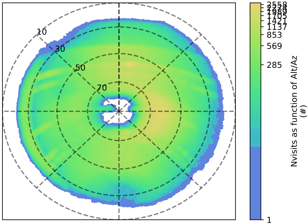
roll_uniform_eh_acc0.2_mjdp0_v3.4_10yrs r: Nvisits as function of Alt/Az
