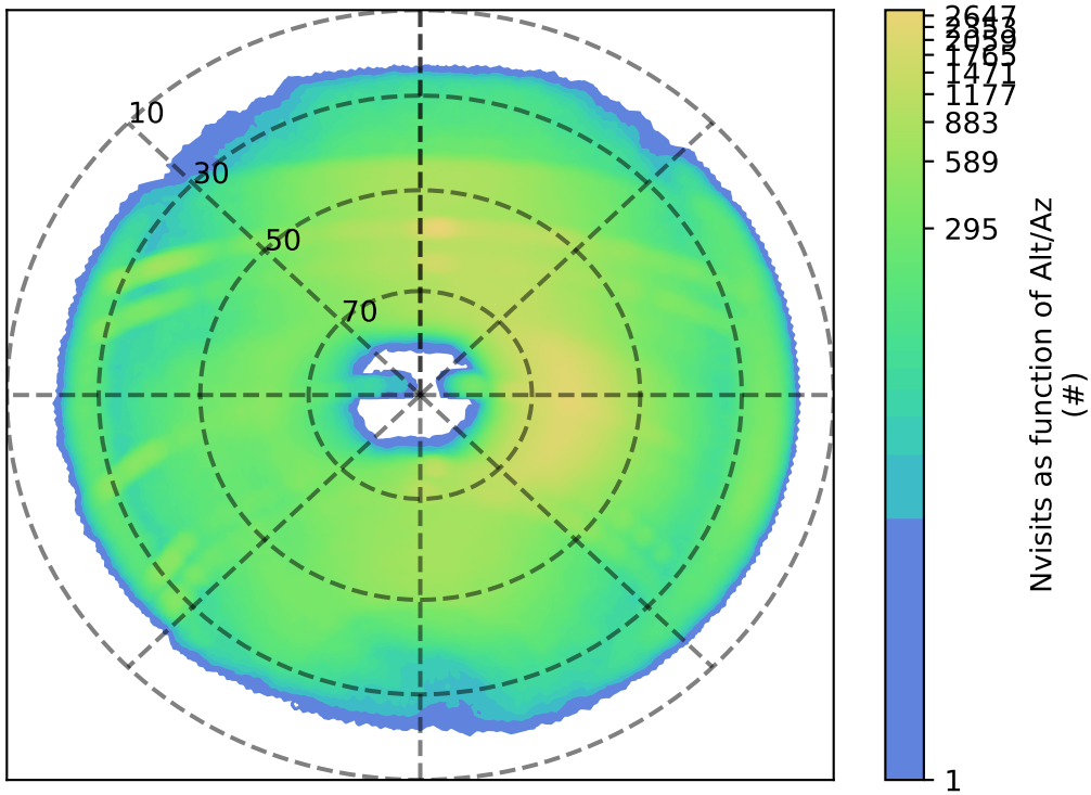
roll_uniform_eh_acc0.2_mjdp0_v3.4_10yrs i: Nvisits as function of Alt/Az
