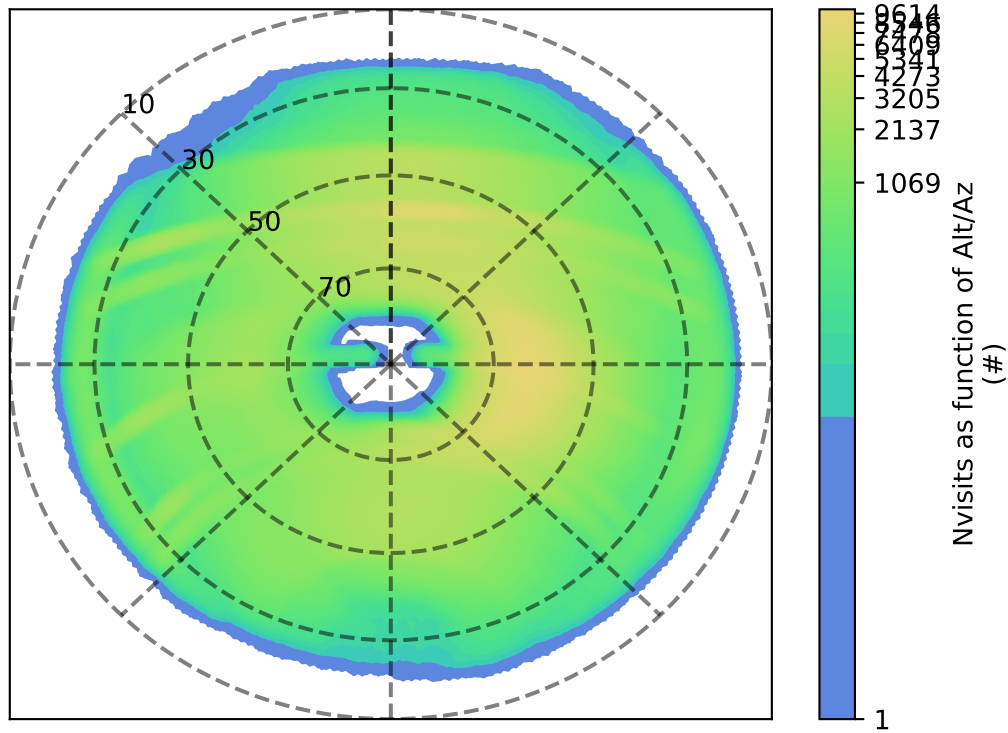
roll_uniform_eh_acc0.2_mjdp0_v3.4_10yrs : Nvisits as function of Alt/Az
