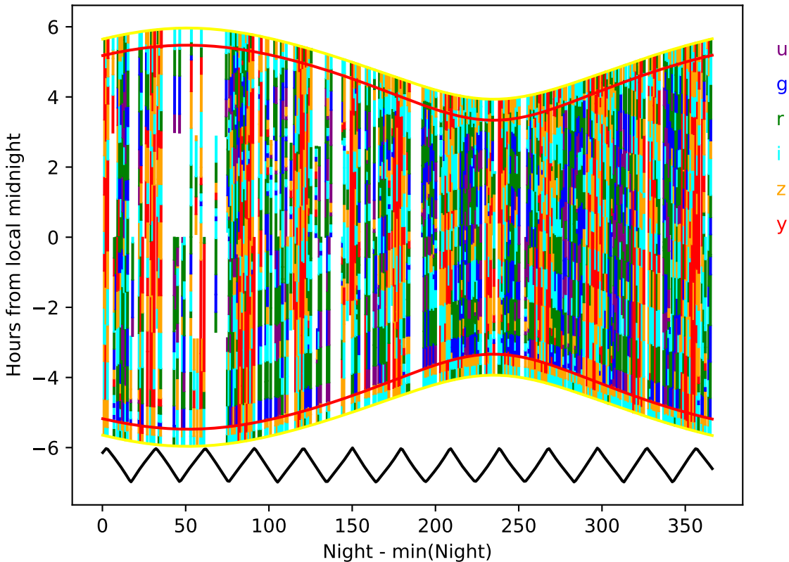
roll_uniform_eh_acc0.2_mjdp0_v3.4_10yrs year 9-10: Hourglass
