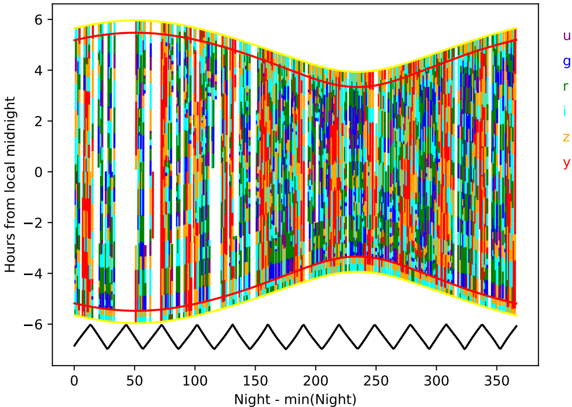
roll_uniform_eh_acc0.2_mjdp0_v3.4_10yrs year 8-9: Hourglass
