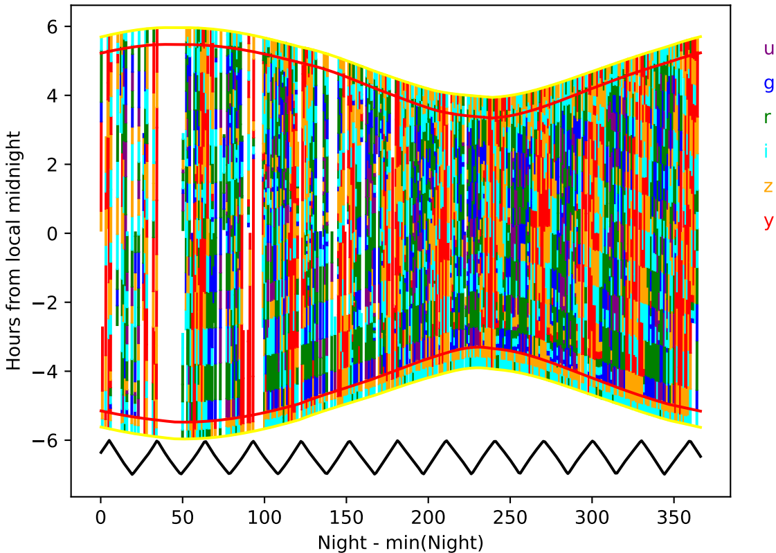
roll_uniform_eh_acc0.2_mjdp0_v3.4_10yrs year 6-7: Hourglass
