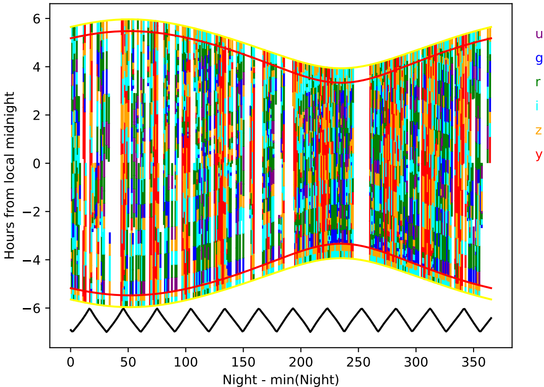
roll_uniform_eh_acc0.2_mjdp0_v3.4_10yrs year 5-6: Hourglass
