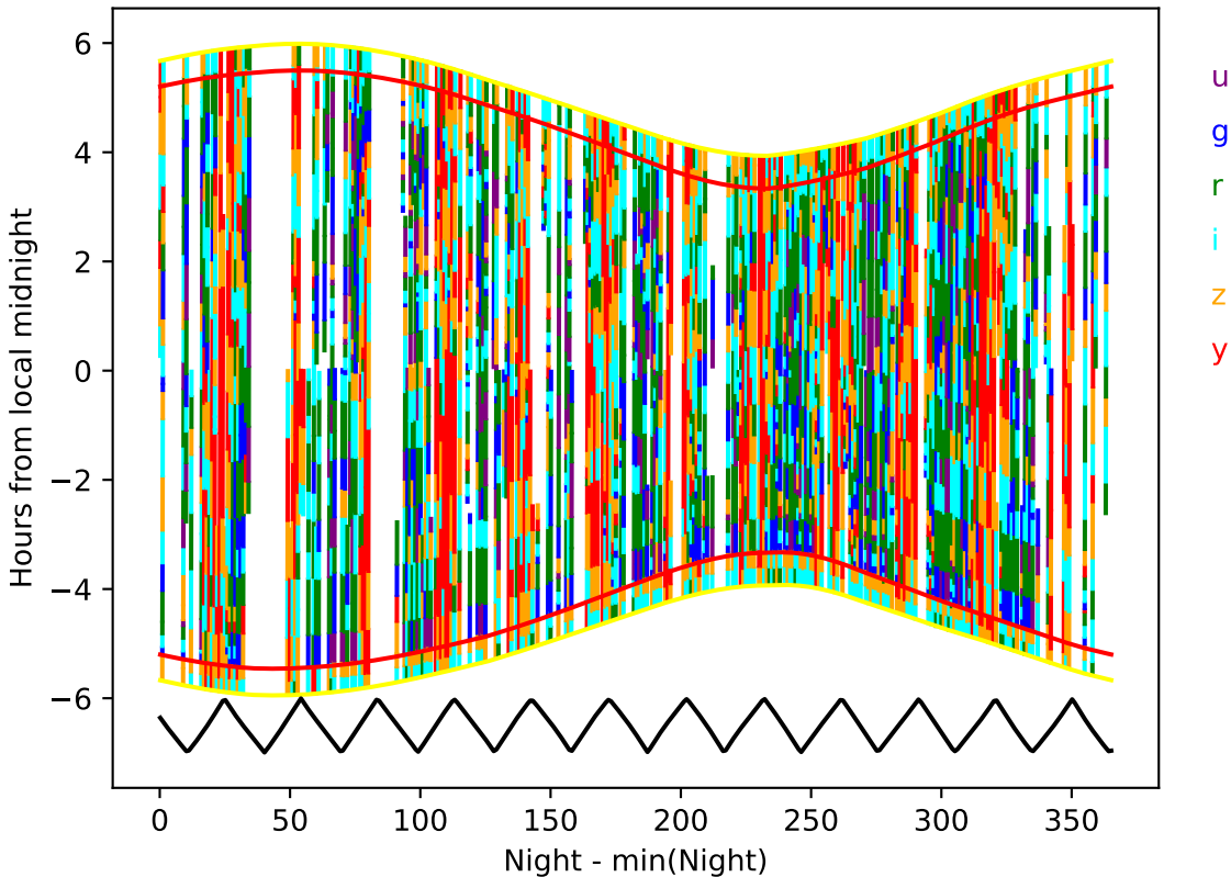
roll_uniform_eh_acc0.2_mjdp0_v3.4_10yrs year 4-5: Hourglass
