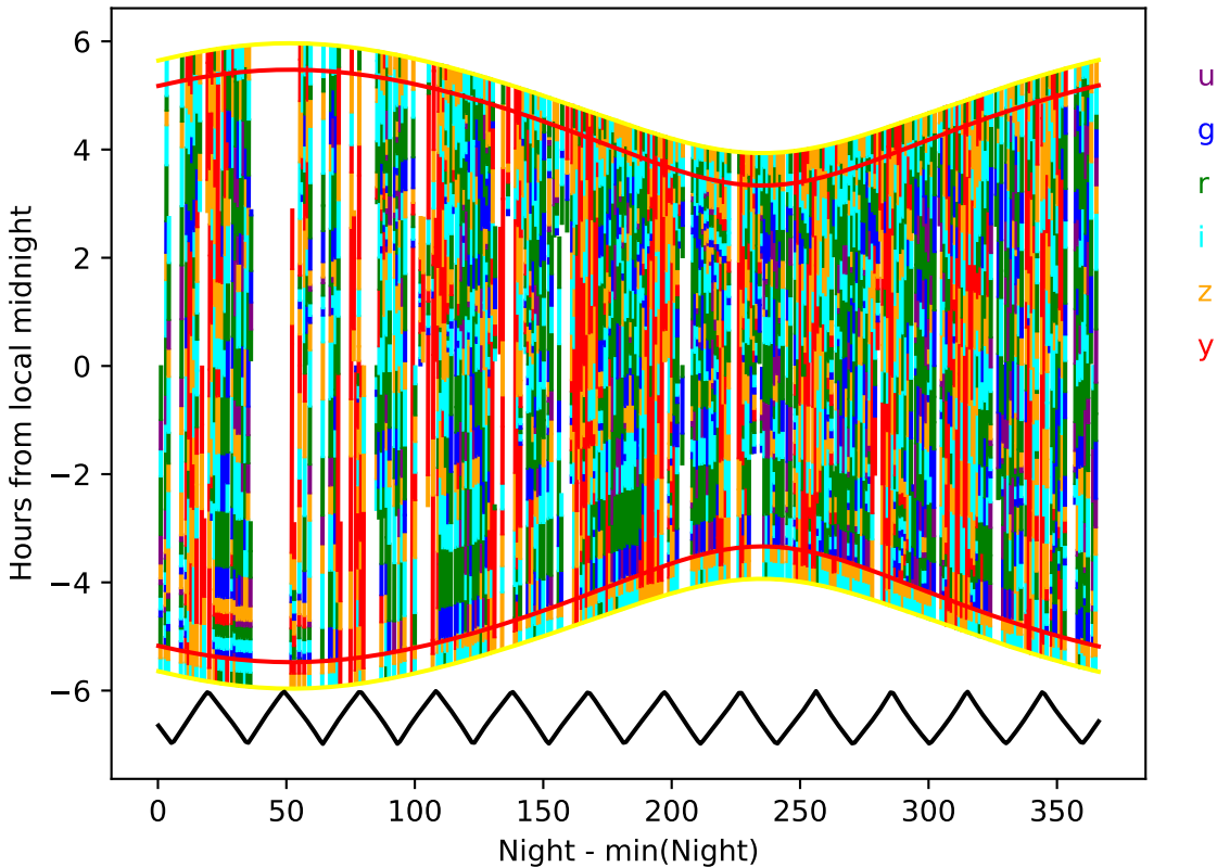
roll_uniform_eh_acc0.2_mjdp0_v3.4_10yrs year 2-3: Hourglass
