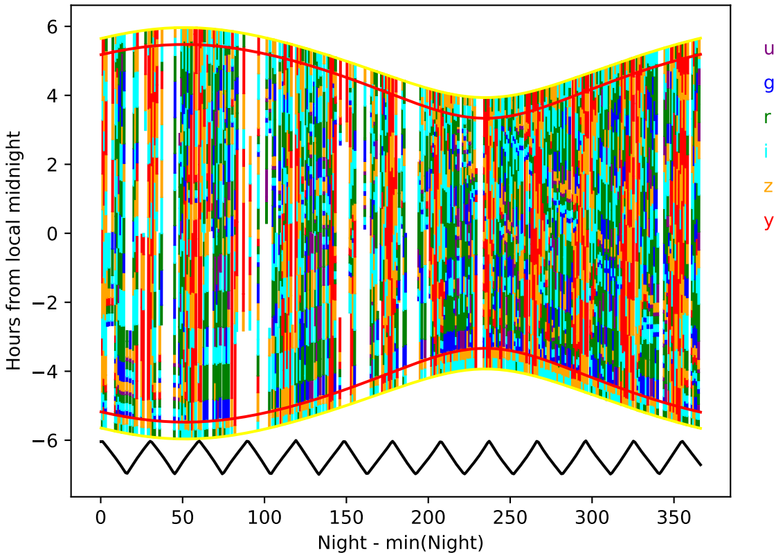
roll_uniform_eh_acc0.2_mjdp0_v3.4_10yrs year 1-2: Hourglass
