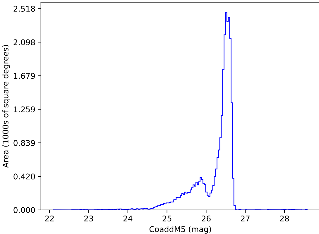
roll_uniform_eh_acc0.2_mjdp0_v3.4_10yrs i: CoaddM5
