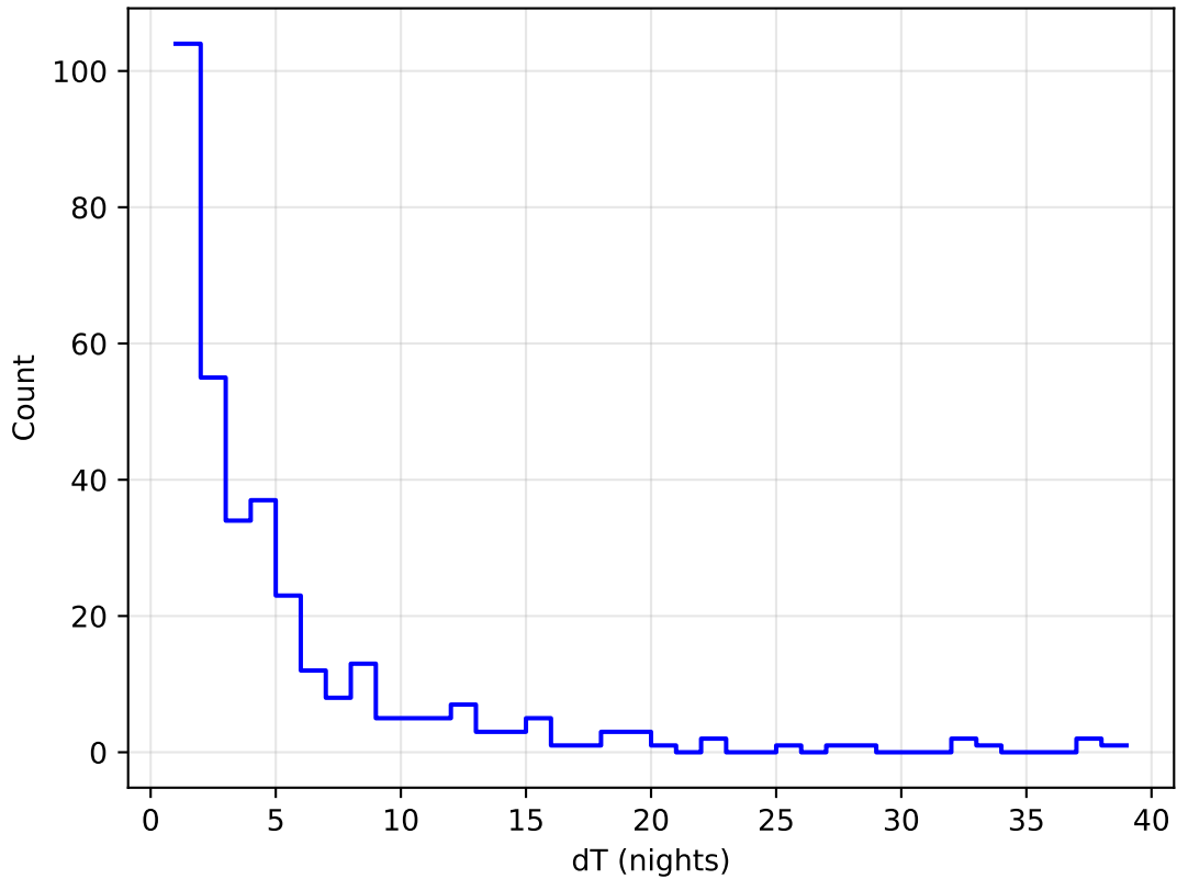
roll_uniform_eh_acc0.2_mjdp0_v3.4_10yrs all bands: DD:WFD Delta Nights Histogram
