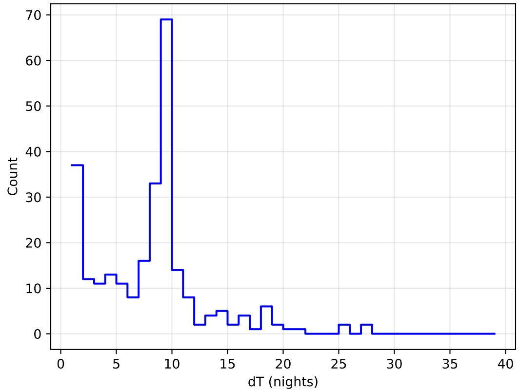
roll_uniform_eh_acc0.2_mjdp0_v3.4_10yrs all bands: DD:ELAISS1 Delta Nights Histogram
