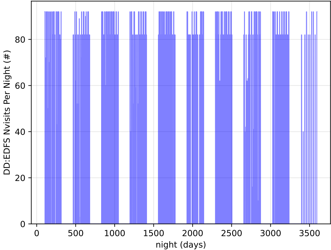
roll_uniform_eh_acc0.2_mjdp0_v3.4_10yrs all bands: DD:EDFS Nvisits Per Night
