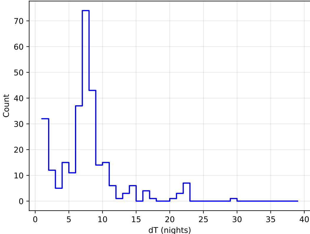
roll_uniform_eh_acc0.2_mjdp0_v3.4_10yrs all bands: DD:EDFS Delta Nights Histogram
