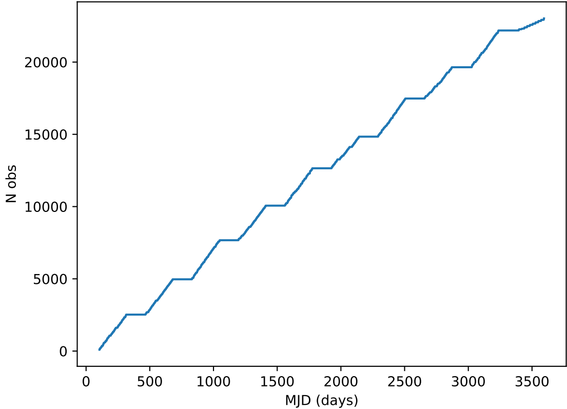
roll_uniform_eh_acc0.2_mjdp0_v3.4_10yrs all bands: DD:EDFS Cumulative NVisits
