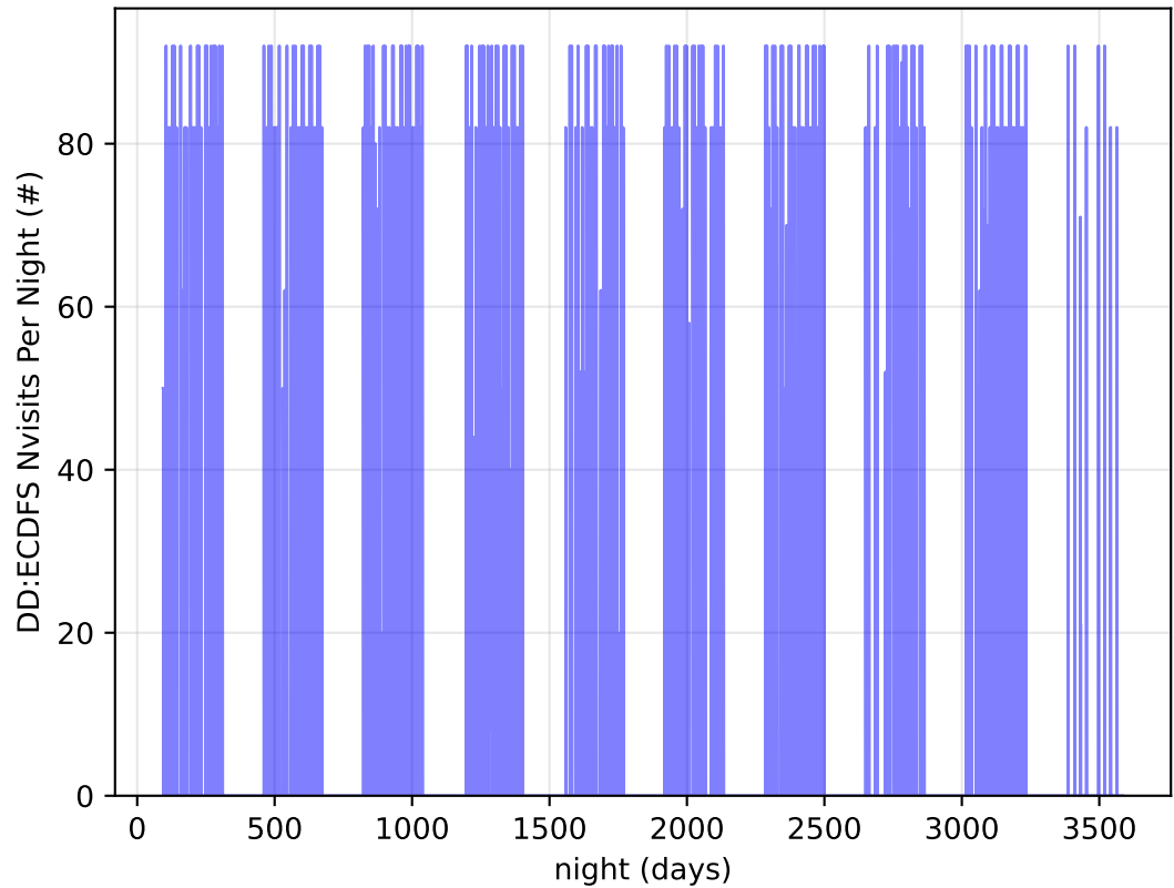
roll_uniform_eh_acc0.2_mjdp0_v3.4_10yrs all bands: DD:ECDFS Nvisits Per Night
