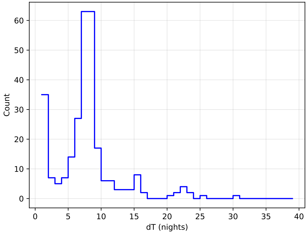
roll_uniform_eh_acc0.2_mjdp0_v3.4_10yrs all bands: DD:ECDFS Delta Nights Histogram
