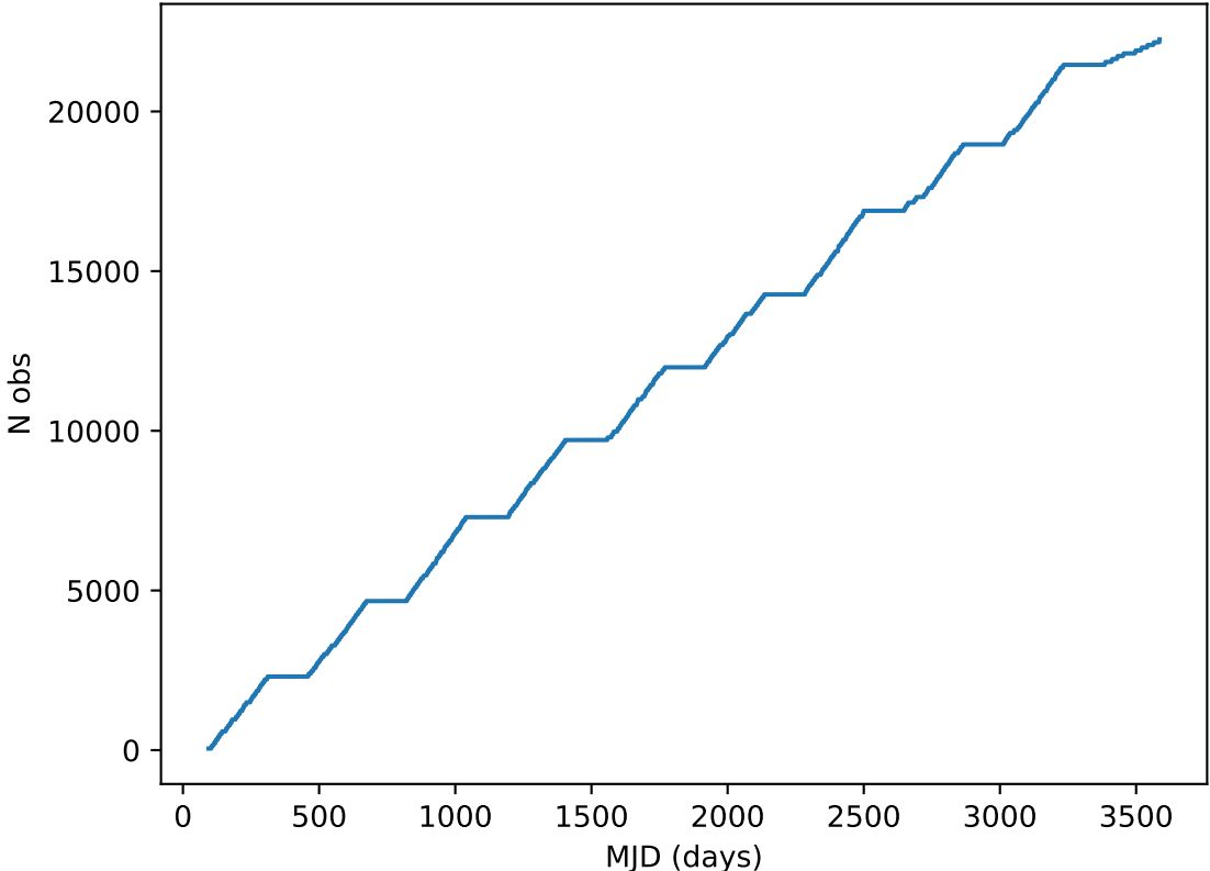
roll_uniform_eh_acc0.2_mjdp0_v3.4_10yrs all bands: DD:ECDFS Cumulative NVisits
