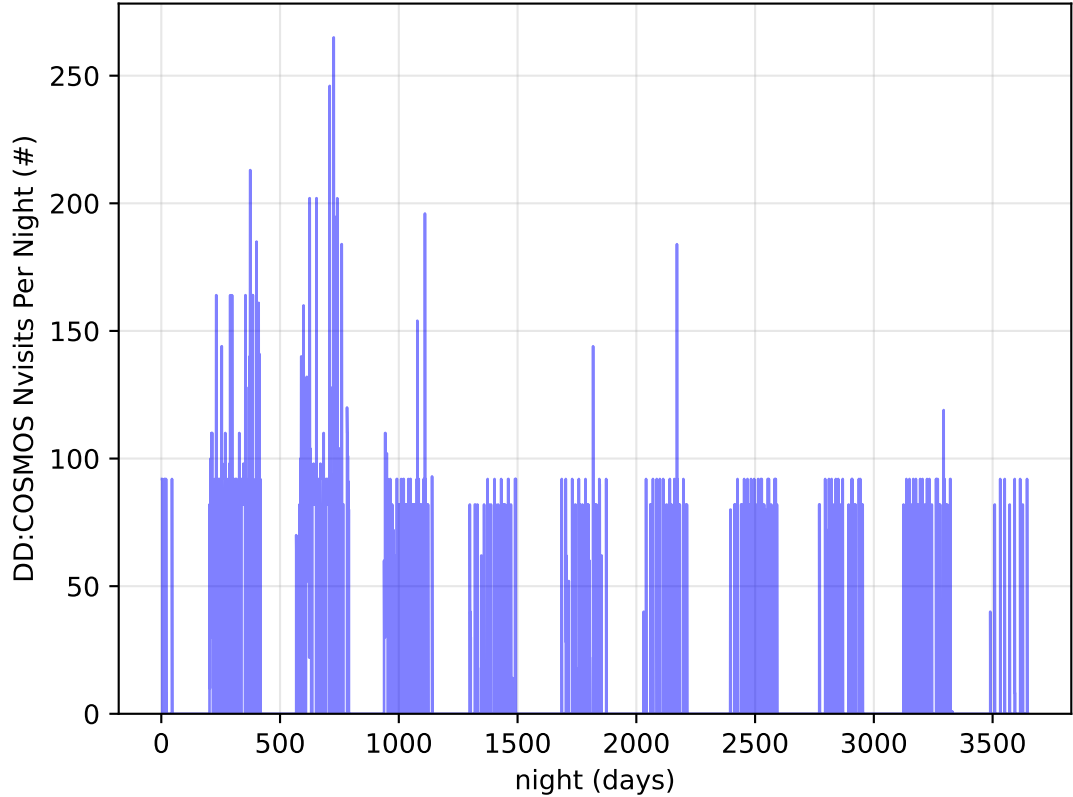
roll_uniform_eh_acc0.2_mjdp0_v3.4_10yrs all bands: DD: COSMOS Nvisits Per Night
