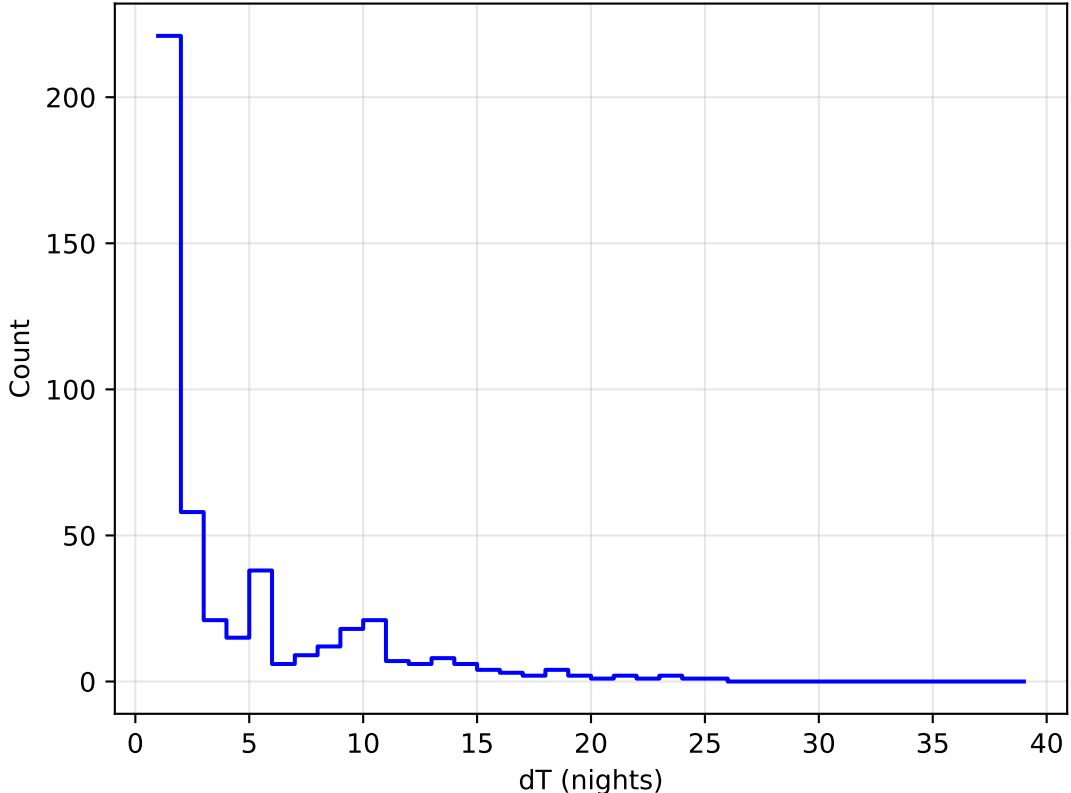
roll_uniform_eh_acc0.2_mjdp0_v3.4_10yrs all bands: DD: COSMOS Delta Nights Histogram
