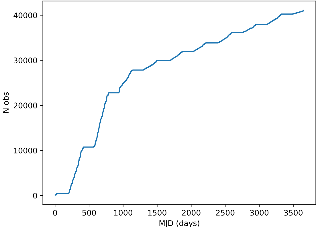
roll_uniform_eh_acc0.2_mjdp0_v3.4_10yrs all bands: DD: COSMOS Cumulative NVisits
